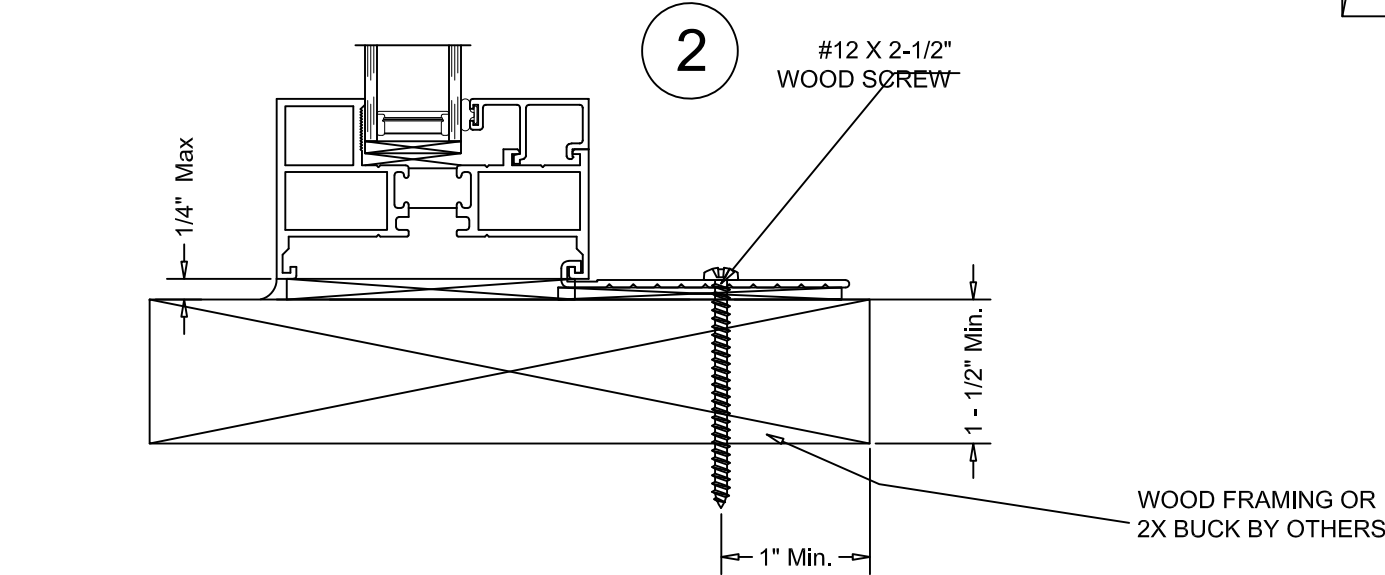
VERTICAL SECTION DETAIL
