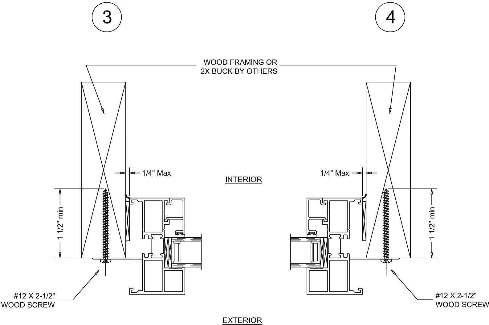
HORIZONTAL SECTION DETAIL WOOD FRAMING INSTALLATION
